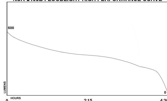
NSR-2168B FLOODLIGHT HIGH PERFORMANCE CURVE
