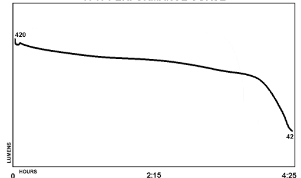
9746 PERFORMANCE CURVE
