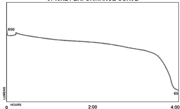
9746XL PERFORMANCE CURVE
