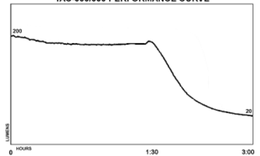
TAC-500/550 PERFORMANCE CURVE
