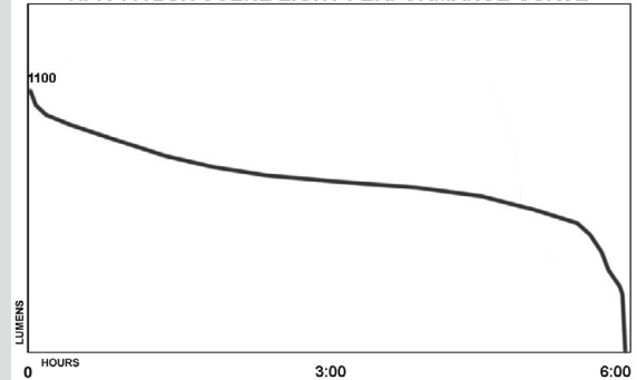
XPR-5592GX SCENE LIGHT PERFORMANCE CURVE
